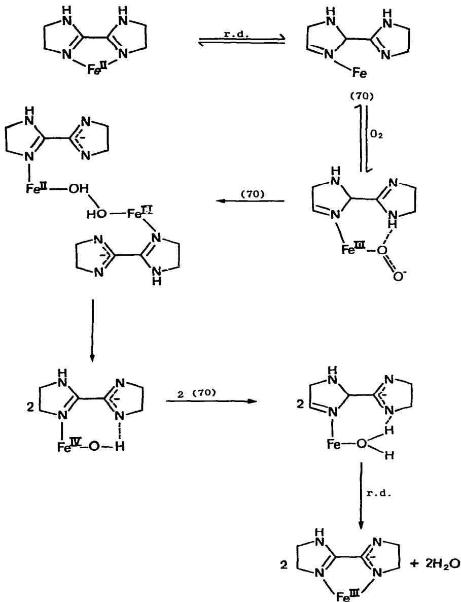
SCHEME XV: The reaction of [\text{Fe}(\text{BlmH})_3]^{2+} with \text{O}_2 (rd = rate determining step).
