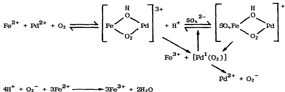
SCHEME VI: The mechanism for the oxidation of [\text{Fe}(\text{H}_2\text{O})_6]^{2+} by \text{O}_2 in the presence of \text{Pd}(\text{II}) .
