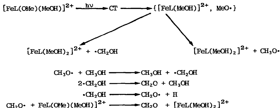
SCHEME VII: Mechanism for the photooxidation of coordinated methanol.
